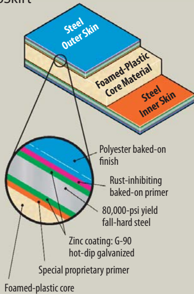
DuraPlate Panel
